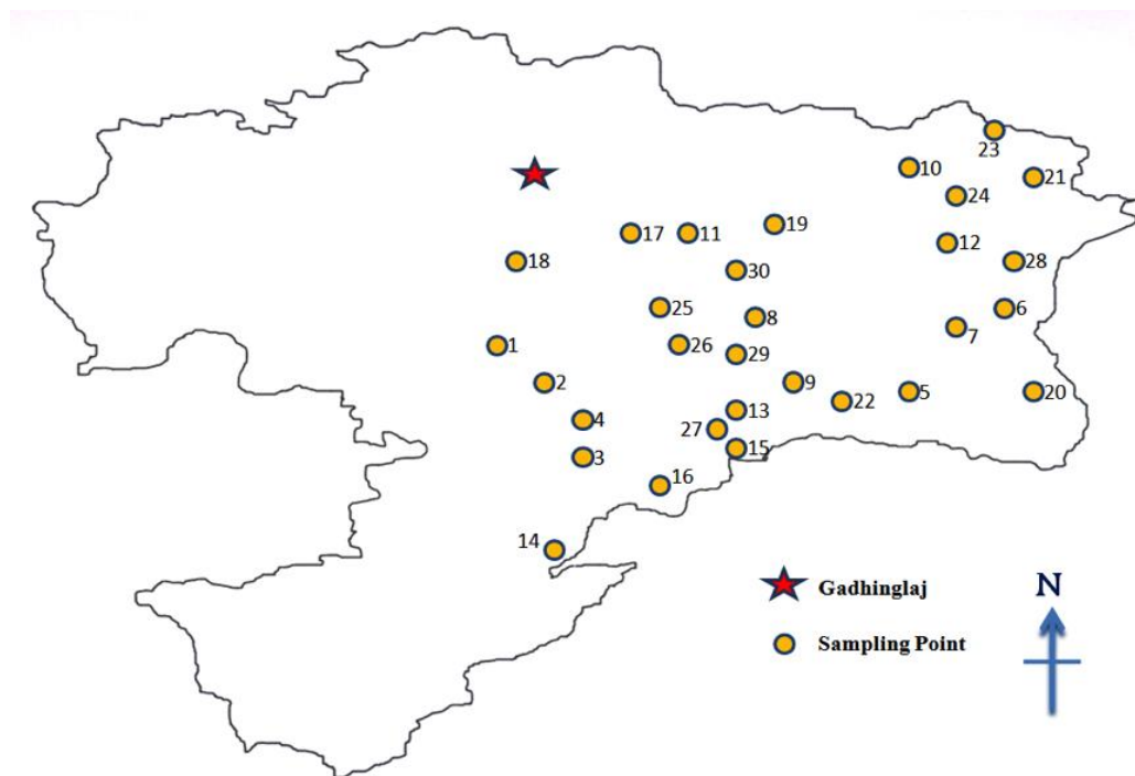
Figure-1. Study area: Sampling sites
